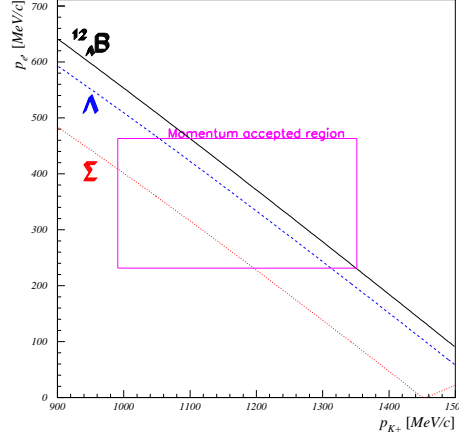
FIGURE 4.40: ENGE AND HKS MOMENTUM CORRELATION. CALCULATED FROM EQN. 4.8 FOR \Lambda , \Sigma AND ^{12}\Lambda B GROUND STATE WITH BEAM ENERGY E_e = 1.853 AND SCATTERING ANGLE VALUES: \theta_{eK^+} = 0.119rad AND \theta_{e'e} = 0.065rad
