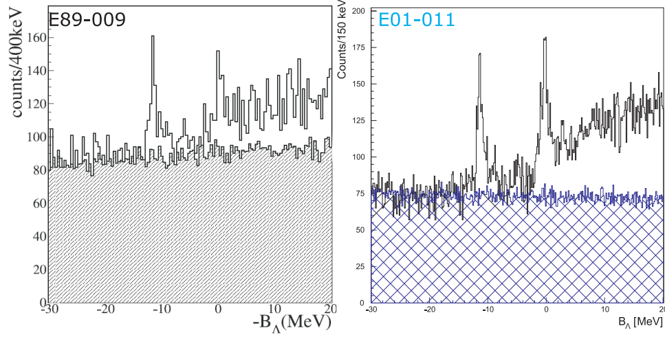
FIGURE 5.4: COMPARISON BETWEEN E89-009 [56] [39] AND E01-011 ^{12}\Lambda B SPECTRA.
