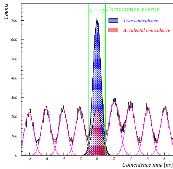
FIGURE 4.2: COINCIDENCE TIME DISTRIBUTION WITH APPLIED KAON PID FOR CH 2 DATA. REAL COINCIDENCE PEAK IS CLEARLY SEEN.
