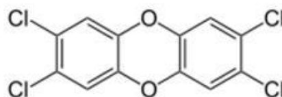
2,3,7,8 - TCDD
