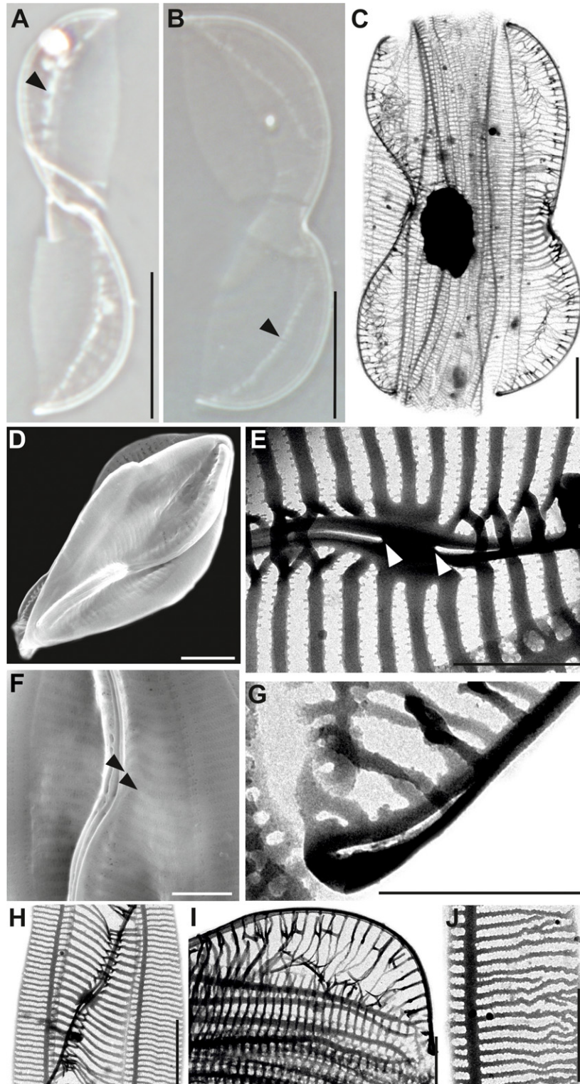
FIG. 6. Entomoneis adriatica sp. nov. Mejdandžić & Bosak. (A, B) LM; (C, E, G–J) TEM; (D, F) SEM. (B–J) strain BIOTAI–49; (A) Natural material (A) Valve in valve view with acute valve apices and distinct basal fibulae (arrowheads). (B) Valve in girdle view with an arcuate transition between the keel and valve body formed by basal fibulae (arrowheads). (C) Frustule in girdle view with straight appearance of the girdle. (D) Twisted cell. (E) Central part of the valve with straight central raphe endings (arrowheads). (F) Double raphe canal (arrowheads) in malformed cell in a prolonged culture. (G) Acute valve apex with straight terminal raphe end. (H) Central part of the valve with attached valvocopula. (I) Terminal part of the cell with distinct basal fibulae forming transition between the keel and valve body. (J) Detail of a valvocopula with bifurcated striae. Scale bars: (A, B) 10 \mu\text{m} ; (C) 5 \mu\text{m} ; (D, H) 2 \mu\text{m} ; (E–G, I, J) 1 \mu\text{m} . [Color figure can be viewed at wileyonlinelibrary.com ]
