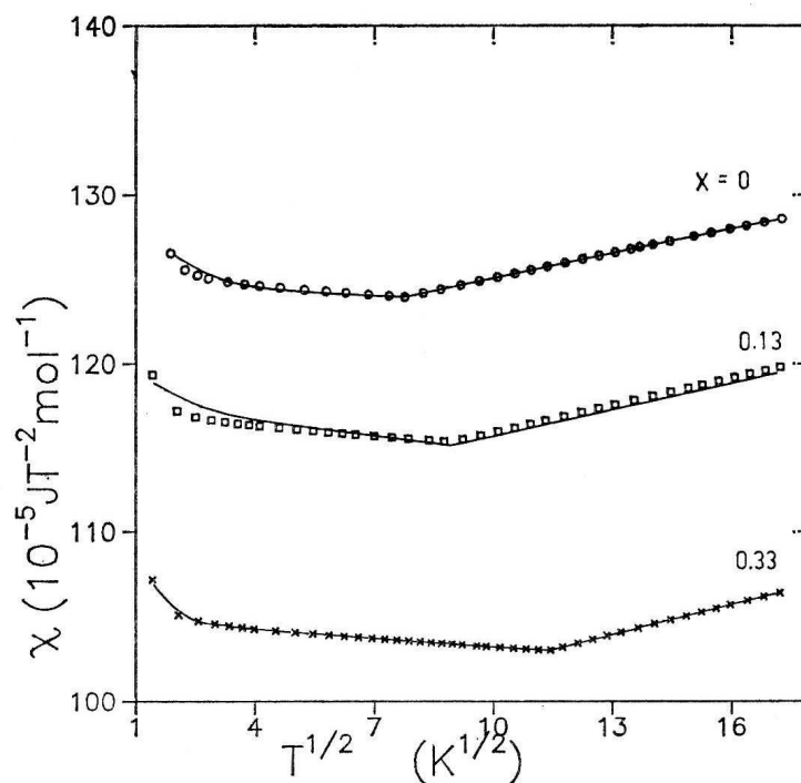
Fig. 6. The magnetic susceptibility of hydrogen doped Zr_{0.67}Ni_{0.33}H_x metallic glasses as a function of the square-root of temperature. The lines are the best fits obtained from Eqs. (20) and (21).
