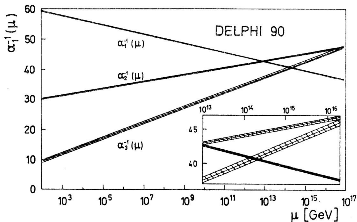
Fig. 3. Recent experiments rule out the simple SU(5) grand unification.
