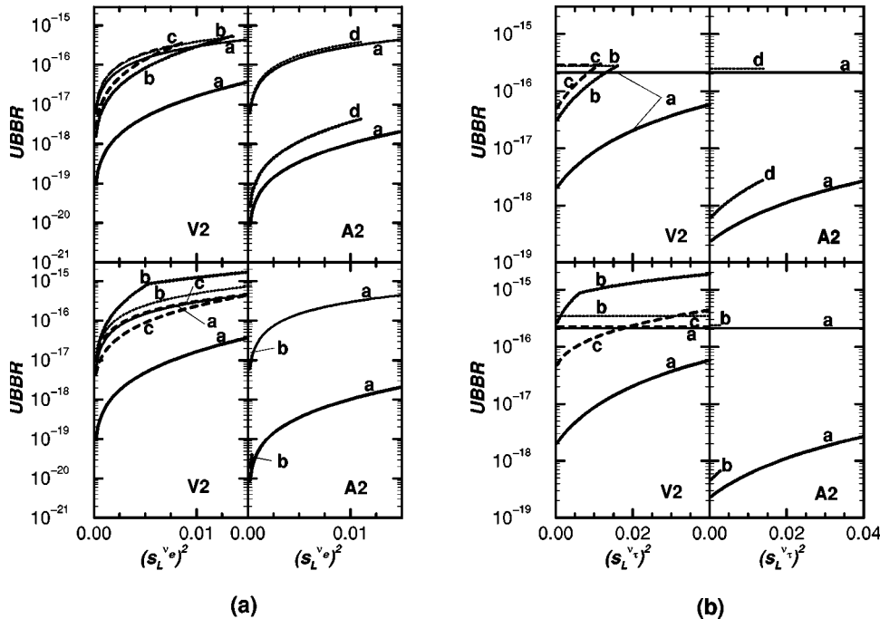
FIG. 5. The UBBRs for K_L \rightarrow e\mu and \pi^0 \rightarrow e\mu decays versus (s_L^{\nu_e})^2 and (s_L^{\nu_\tau})^2 for several m_{N_1} values and several \rho_2 values in models V2 and A2.
