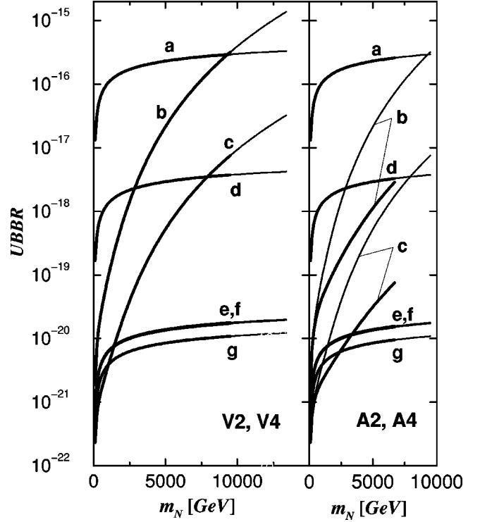
FIG. 1. The UBBRs for the most interesting LFV hadron decays versus m_N = m_{N_i} , i=1, n_R in models V2, V4, A2, and A4.
