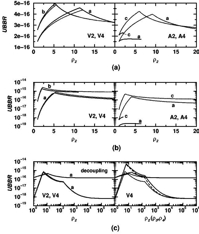
FIG. 4. The UBBRs for K_L \rightarrow e\mu and \pi^0 \rightarrow e\mu decays versus ratios \rho_i = m_{N_i}/m_N for several m_{N_1} values in models V2, V4, A2, and A4.
