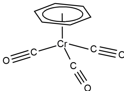
b) [\text{Cr}(\eta^6\text{-C}_6\text{H}_6)(\text{CO})_3]
