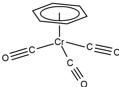
b) [\text{Cr}(\eta^6\text{-C}_6\text{H}_6)(\text{CO})_3]
