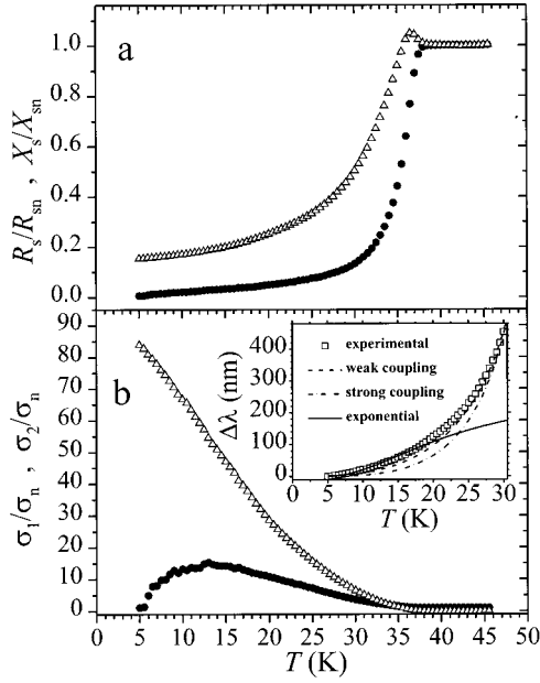
FIG. 3. (a) Plot of R_s/R_{sn} (solid circles) and X_s/X_{sn} (open up triangles) against temperature. (b) The corresponding \sigma_1/\sigma_n (solid circles) and \sigma_2/\sigma_n (open up triangles) plotted against temperature. The data are normalized to the values at 40 K. The inset shows the temperature variation of the London penetration depth \Delta\lambda(T) . The dashed line is the function given by Eq. (3) with \lambda_0=800 nm and n=3-T/T_c for the weak-coupling case, while the dash-dotted line represents the strong-coupling case ( n=4 ) with \lambda_0=1600 nm. The solid line is exponential behavior given by Eq. (4) with \Delta/kT_c=1.05 and \lambda_0=450 nm.
