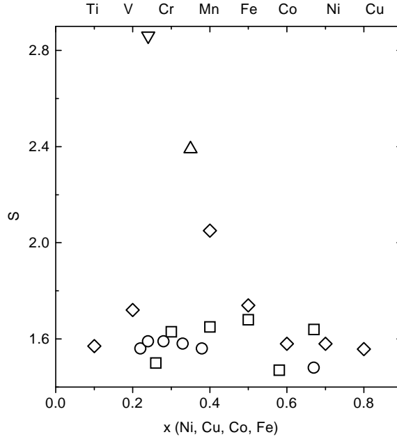
Fig. 2. The Stoner factor of Zr_{1-x}Cu_x (□), Zr_{1-x}Ni_x (○), Zr_{1-x}Co_x (△), Zr_{1-x}Fe_x (▽) alloys versus x (bottom scale), and Zr_2(Ni_{0.9}M_{0.1})_1 (◇) alloys versus M (top scale).
