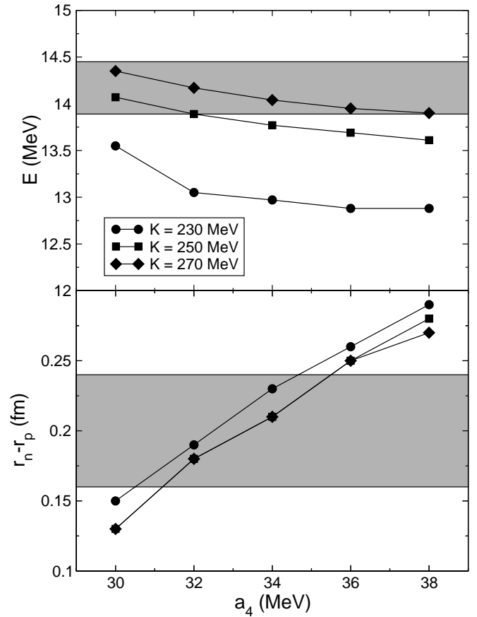
FIG. 5. The RRPA excitation energies of the GMR in ^{208}\text{Pb} as functions of the volume asymmetry a_4 , calculated for the three sets of interactions with K_{\text{nm}}=230, 250, and 270 MeV. The theoretical centroids are shown in comparison with the experimental excitation energy of the monopole resonance: E=14.17 \pm 0.28 MeV [4]. In the lower panel, the corresponding results for the difference of the neutron and proton radii in ^{208}\text{Pb} are plotted in comparison with the experimental value 0.20 \pm 0.04 fm [27].
