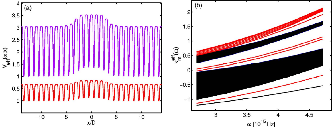
FIG. 1. (Color online) The effective potentials and band gap structure at different temporal frequencies. (a) The effective potential V_{\text{eff}}(\omega; x) for \lambda = 400 nm (violet line) and \lambda = 700 nm (red line) of the self-consistently calculated IWLLS (the potential value for the violet light is shifted upwards by 1 for better comparison). (b) The band gap structure of the lattice (shaded regions denote bands), and the effective propagation constants \kappa_m^{\text{eff}}(\omega) of the populated soliton modes (red lines).
