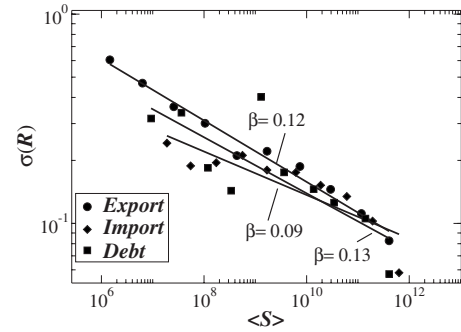
FIG. 1. Standard deviation \sigma(R) of the logarithmic growth rate R as a function of the average value S of imports, exports, and debt. We find that, for each of the three economic variables, the standard deviation \sigma(R) decays algebraically with S . Interestingly, all three scaling exponents \beta are similar to each other and surprisingly similar to the scaling exponent \beta \approx 0.15 observed for the gross domestic product of countries (GDP) and firms.
