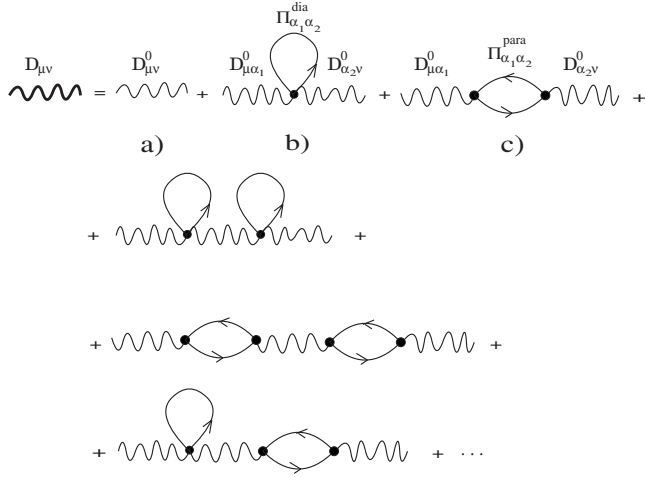
FIG. 2. Perturbation expansion for the photon propagator D_{\mu\nu} .
