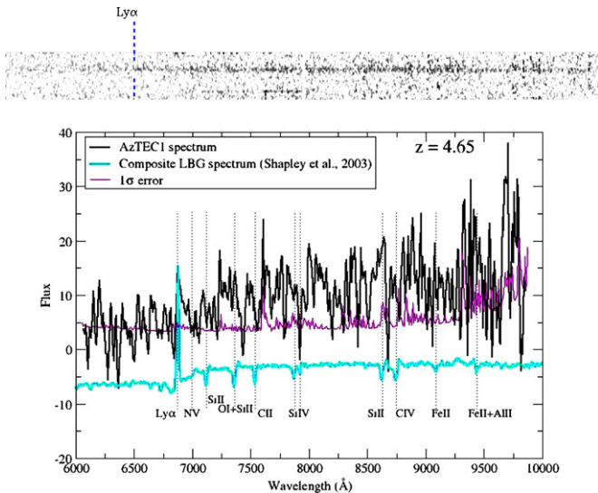
Figure 2. Top panel shows the Keck II/DEIMOS 2D spectrum of AzTEC 1. Note the increase in continuum flux beyond Ly \alpha (see also Figure 3). In the bottom panel the extracted 1D spectrum is shown. Note that the atmospheric B band (6860–6890 Å) is coincident with the expected Ly \alpha emission line. The composite LBG spectrum is from Shapley et al. (2003).
