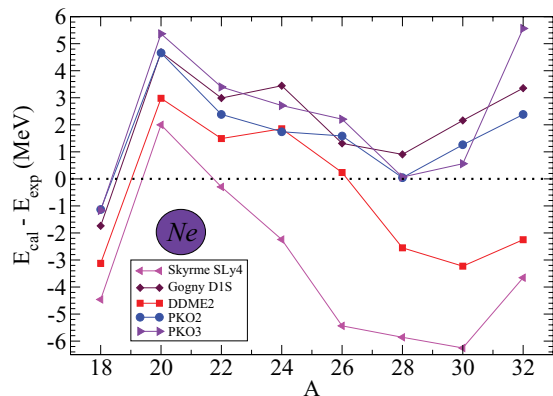
FIG. 9. (Color online) Same as in Fig. 4, but with the PKO3 RHFb calculation in addition.
