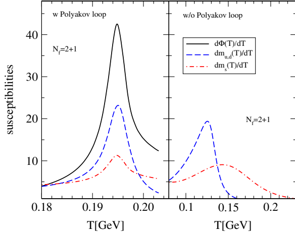
FIG. 1 (color online). (Color online) Quark-mass susceptibilities (blue dashed line: light flavors; red dash-dotted line: strange flavor) with coupling to the Polyakov loop (left panel) and without it (right panel) as a function of the temperature. Note that without coupling to the Polyakov loop the chiral transition temperature is unrealistically low and the peak value for the light flavors is different from that for the strange one.
