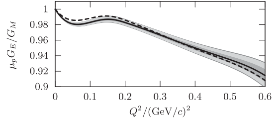
FIG. 2. \mu_p G_E/G_M with Coulomb correction as published (solid), with TPE according to Borisjuk and Kobushkin (dashed).
