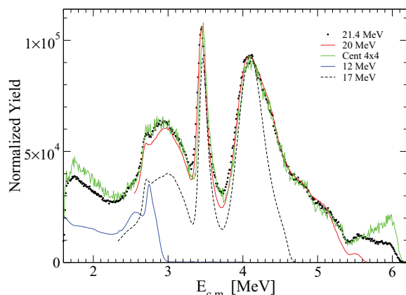
FIG. 2. (Color online) The excitation function for ^9\text{Be} + \alpha measured at 21.4 MeV (black dots), 20 MeV (red line), 17 MeV (dashed line), and 12 MeV (blue line). The 21.4 MeV data restricted to the central 4 \times 4 pixels are shown by the green line.
