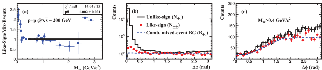
FIG. 5. (Color online) (a) The ratio of like-sign to mixed-event distributions in minimum-bias p + p collisions. (b) The distribution of the difference of the azimuthal angles ( \Delta\phi ) of the two electrons in the unlike-sign, like-sign, and mixed-event pairs in minimum-bias p + p collisions. (c) The \Delta\phi distributions of unlike-sign, like-sign, and mixed-event pairs for M_{ee} > 0.4 GeV/c 2 in minimum-bias p + p collisions. Errors are statistical.
