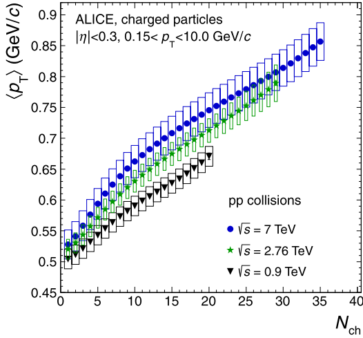
Fig. 1. Average transverse momentum \langle p_T \rangle in the range 0.15 < p_T < 10.0 GeV/c as a function of charged-particle multiplicity N_{ch} in pp collisions at \sqrt{s} = 0.9, 2.76, and 7 TeV, for |\eta| < 0.3 . The boxes represent the systematic uncertainties on \langle p_T \rangle . The statistical errors are negligible.
