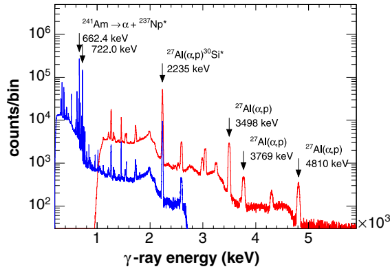
FIG. 3. (Color online) The \gamma -ray spectrum of the ^{241}\text{Am} measured in two energy ranges with a HPGe setup [46]. Some characteristic \gamma rays from \alpha decay or from \alpha induced reactions are shown as well.
