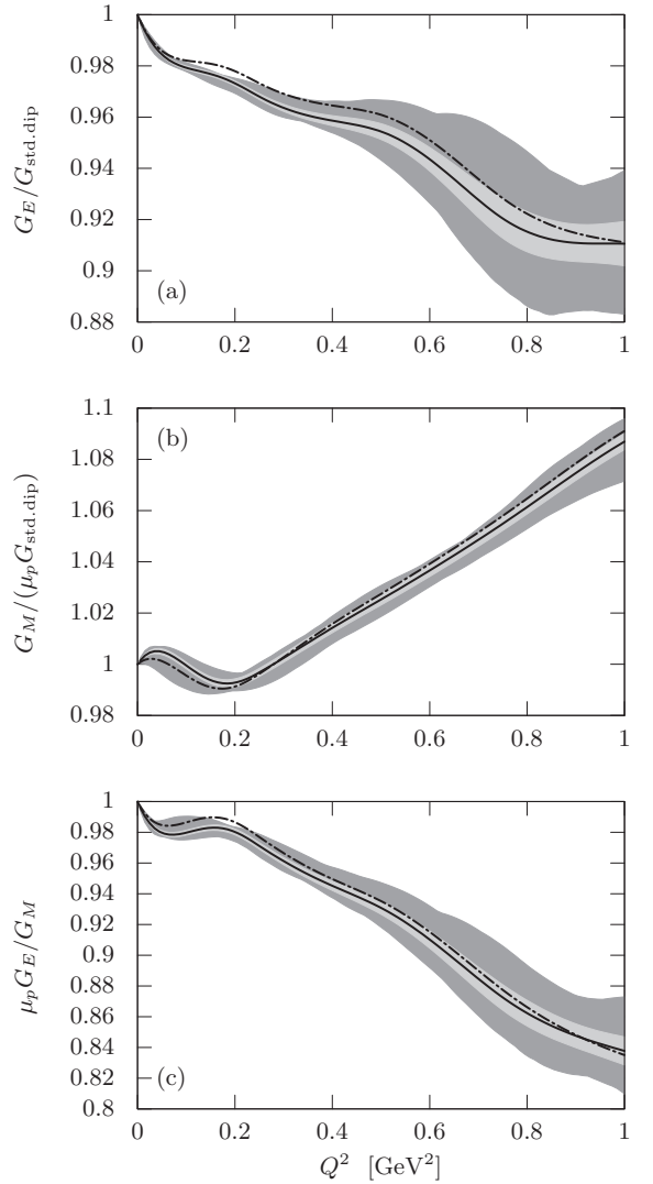
FIG. 20. The spline fit with variable knots from Fig. 14, zoomed in to Q^2 < 1 (\text{GeV}/c)^2 . The dashed-dotted line represents a fit of all data up to 5(\text{GeV}/c)^2 , with TPE corrections according to Refs. [97–99] applied.
