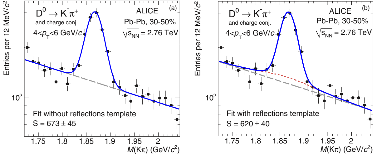
FIG. 5. (Color online) Invariant mass distribution of D^0 candidates with 4 < p_T < 6 GeV/ c in the centrality class 30%–50%: (a) fit without template for reflections and (b) with template for reflections (dotted line). The raw yield obtained as an integral of the signal Gaussian function is reported.
