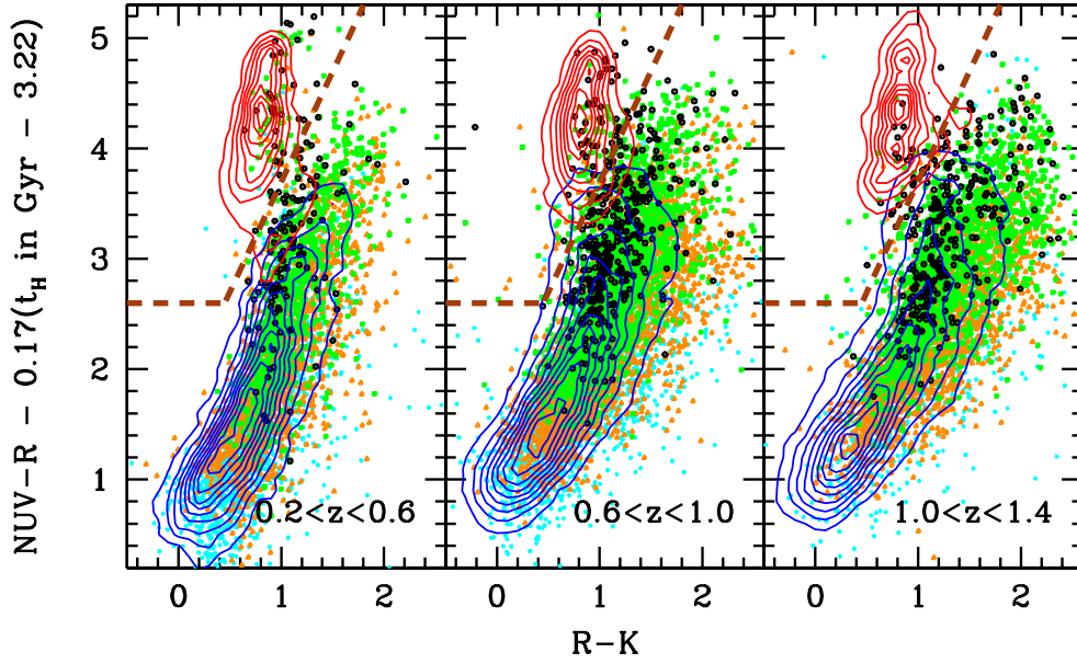
Fig. 2. NUV - R - 0.17(t_H \text{ in Gyr} - 3.22) versus R - K rest-frame colors in the COSMOS field at 0.2 < z < 1.4 and \log(M_*/M_\odot) > 9.5 . An additional term depending on the redshift is added to the NUV - R color in order to keep the same criterion to separate quiescent and star-forming galaxies valid at all redshifts (brown dashed lines). Cyan crosses, orange triangles, green squares and black circles correspond to galaxies with masses at \log(M_*) = 9.5-10 , 10-10.5 , 10.5-11 and 11-11.5 , respectively. The red and blue contours indicate the distribution of the mass selected galaxies ( \log(M_*/M_\odot) > 9.5 ) with \log(sSFR)_{\text{SED}} < -2 and \log(sSFR)_{\text{SED}} > -2 , respectively.
