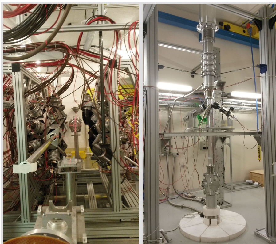
Fig. 4. Picture of the horizontal neutron beam line in EAR1 (left panel) showing the TAC in open position, and the vertical neutron beam line in the newly constructed EAR2 (right panel), showing a neutron capture setup with C_6D_6 detectors above the chamber containing the silicon neutron beam monitors (SiMon2).
