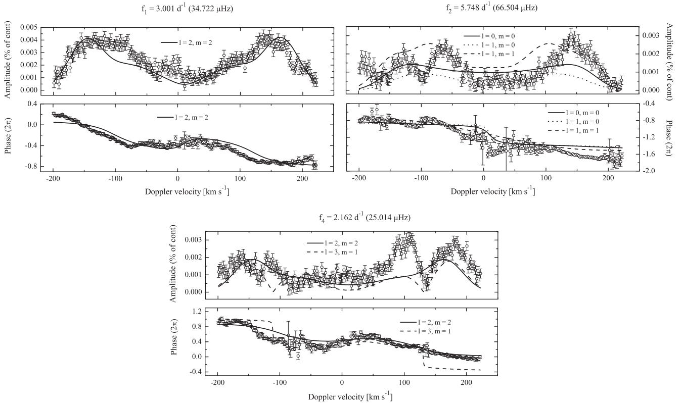
Figure 9. Amplitude and phase distributions across the line profile for three pulsations modes: f_1 = 3.001 \text{ d}^{-1} (top left), f_2 = 5.748 \text{ d}^{-1} (top right), and f_4 = 2.162 \text{ d}^{-1} (bottom). The best-fitting models are overlotted with the lines of different style; the corresponding mode geometry is indicated in each subplot.
