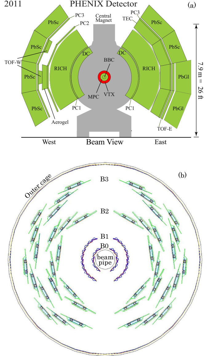
FIG. 1. (a) A schematic view of the PHENIX detector configuration for the 2011 run. (b) A schematic view of the VTX detector with the individual ladders shown.
