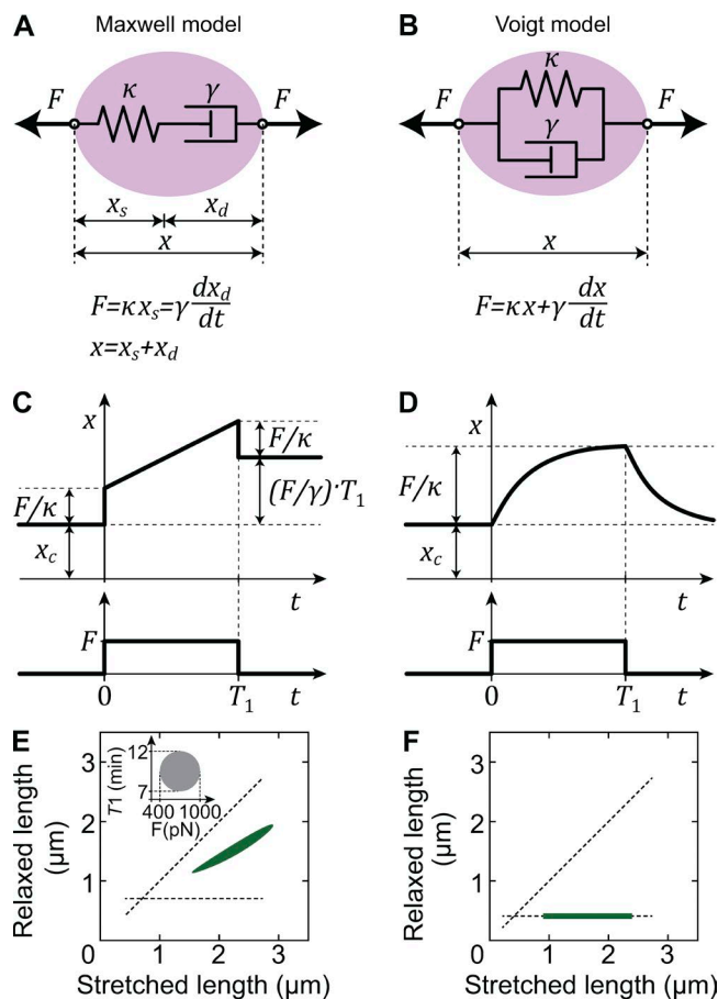
Figure 5. Two simple models of a KT as a viscoelastic object consisting of a spring and a dashpot. (A and B) Schematic representation of the models. A spring of a stiffness \kappa and a dashpot of a viscous drag coefficient \gamma are connected in series (A) or in parallel (B). The KT (pink ellipse) is under tension F and has a length x . In A, the length is the sum of the length of the spring, x_s , and the length of the dashpot, x_d . The equations of the models are given under the schemes. (C and D) KT length as a function of time for the models in A and B, respectively, for a constant tension F that starts to act at time t = 0 and stops at t = T_1 . The length of a control KT is denoted x_c . (E and F) Relaxed length as a function of the stretched length (dark green) for the models in A and B, respectively. In E, \gamma = 5 \times 10^5 pNs/ \mu\text{m} , \kappa = 1,000 pN/ \mu\text{m} , and x_c = 0.7 \mu\text{m} , whereas F and t were varied simultaneously in the intervals F = 400 – 1,000 pN and T_1 = 7 – 12 min, as shown in the inset. In F, \kappa = 100 pN/ \mu\text{m} , x_c = 0.4 \mu\text{m} , and F was varied in the interval 50 – 200 pN. Horizontal and oblique dashed lines correspond to complete relaxation to the control length x_c and no relaxation, respectively.
