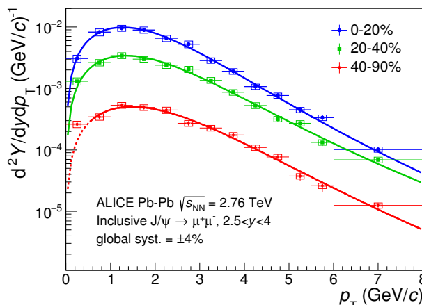
Figure 5. Differential yields of inclusive J/\psi in Pb–Pb collisions at \sqrt{s_{\text{NN}}} = 2.76 TeV as a function of p_{\text{T}} for three centrality classes. Solid lines correspond to the results from the fit described in the text.
