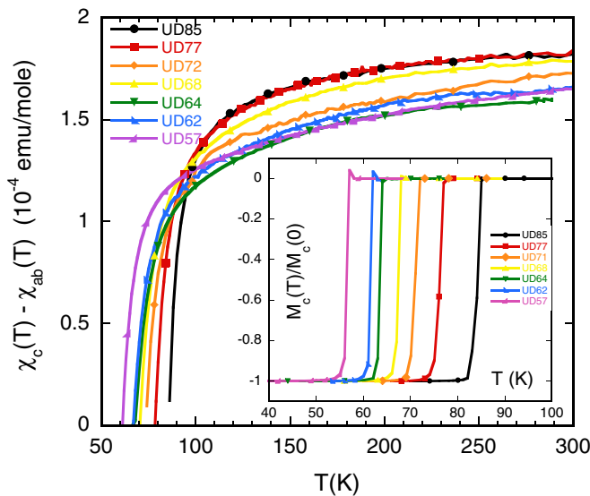
FIG. 3. Susceptibility anisotropy \chi_D(T) = \chi_c(T) - \chi_{ab}(T) for \text{YBa}_2\text{Cu}_3\text{O}_{6+x} single crystals. Inset: Superconducting transitions of the \text{YBa}_2\text{Cu}_3\text{O}_{6+x} crystals for H \parallel c measured on warming in 10 G after zero-field cooling.
