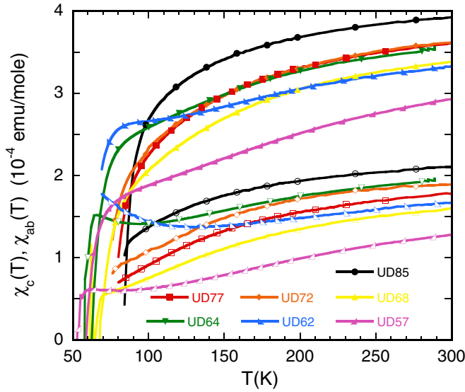
FIG. 2. Temperature dependence of the static magnetic susceptibility \chi_c(T) (full symbols) and \chi_{ab}(T) (empty symbols) for H = 5 \text{ T} \parallel the c axis and the ab plane, respectively.
