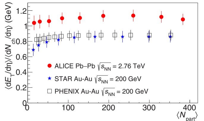
FIG. 10. Comparison of \langle dE_T/d\eta \rangle / \langle dN_{ch}/d\eta \rangle versus \langle N_{part} \rangle at midrapidity in Pb-Pb collisions at \sqrt{s_{NN}} = 2.76 TeV from ALICE and in Au-Au collisions at \sqrt{s_{NN}} = 200 GeV from STAR [29] and PHENIX [26,27].
