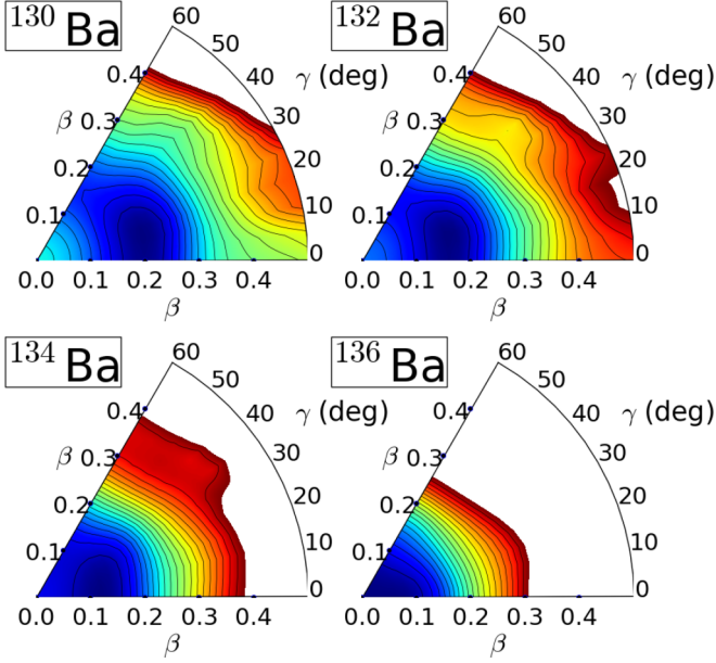
FIG. 1. Self-consistent RHB triaxial quadrupole binding energy maps of the even-even ^{130-136}\text{Ba} isotopes in the \beta - \gamma plane ( 0 \leq \gamma \leq 60^\circ ). For each nucleus the energy surface is normalized with respect to the binding energy of the absolute minimum, and is plotted up to 10 MeV excitation energy with 0.2 MeV difference between neighboring contours.
