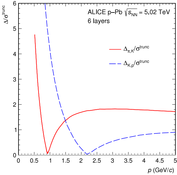
Fig. 40. Measured separation power ( \frac{\Delta}{\sigma^{\text{trunc}}} = \frac{S_{\pi/K}^{\text{trunc}} - S_{\pi/K}^{\text{trunc}}}{\sigma^{\text{trunc}}} ) for \pi/K and K/p separation as a function of momentum.
