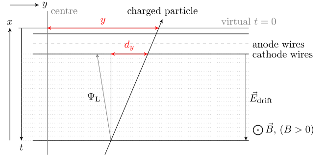
Fig. 46. Sketch of the tracklet reconstruction. The tracklet reconstruction in the MCMs is performed in a local coordinate system. The tracklet comprises the information on y , d_y , z and PID. The magnetic and electric field and the effect of the Lorentz angle ( \Psi_L ) are indicated as well.
