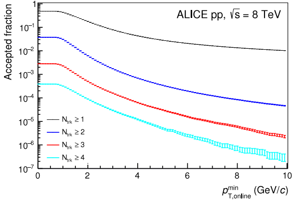
Fig. 54. Rejection by the level-1 trigger for requiring 1–4 tracks in any stack ( N_{trk} ) above varying p_T thresholds for pp collisions at \sqrt{s} = 8 TeV [70]. The error bars indicate the statistical uncertainties. The distributions were obtained by counting the number of tracks in a stack above a given threshold and normalised by the number of sampled events.
