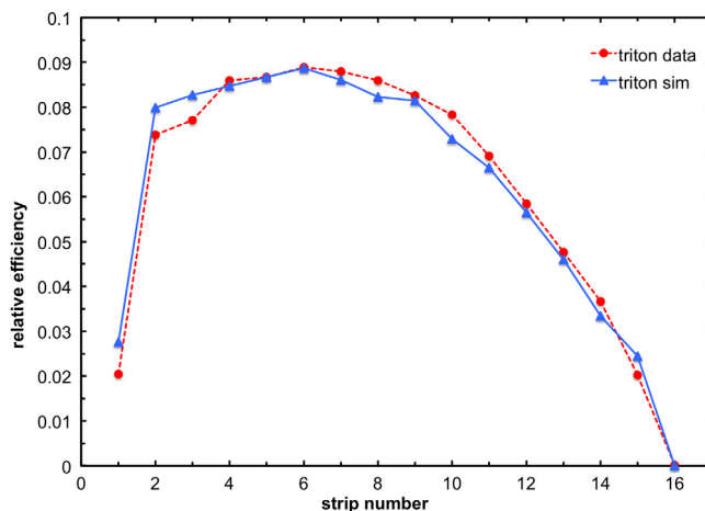
Fig. 6. Detection efficiency of the setup normalized to unity area, as a function of strip number, obtained in the GEANT4 simulation (isotropic emission was assumed) and with ^6\text{LiF} target (triton detection in the validation test).
