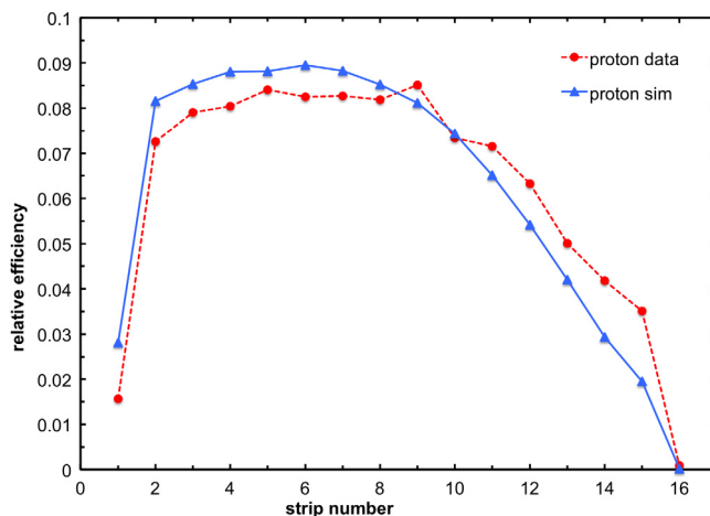
Fig. 7. Detection efficiency of the setup normalized to unity area, as a function of strip number, obtained in the GEANT4 simulation (isotropic emission was assumed) and with ^7\text{Be} target (proton detection).
