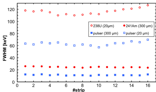
Fig. 4. FWHM resolution for each \Delta E and E detector strip, tested with a pulser and with \alpha particles from ^{238}\text{U} (for the \Delta E detector) and ^{241}\text{Am} (for the E detector).
