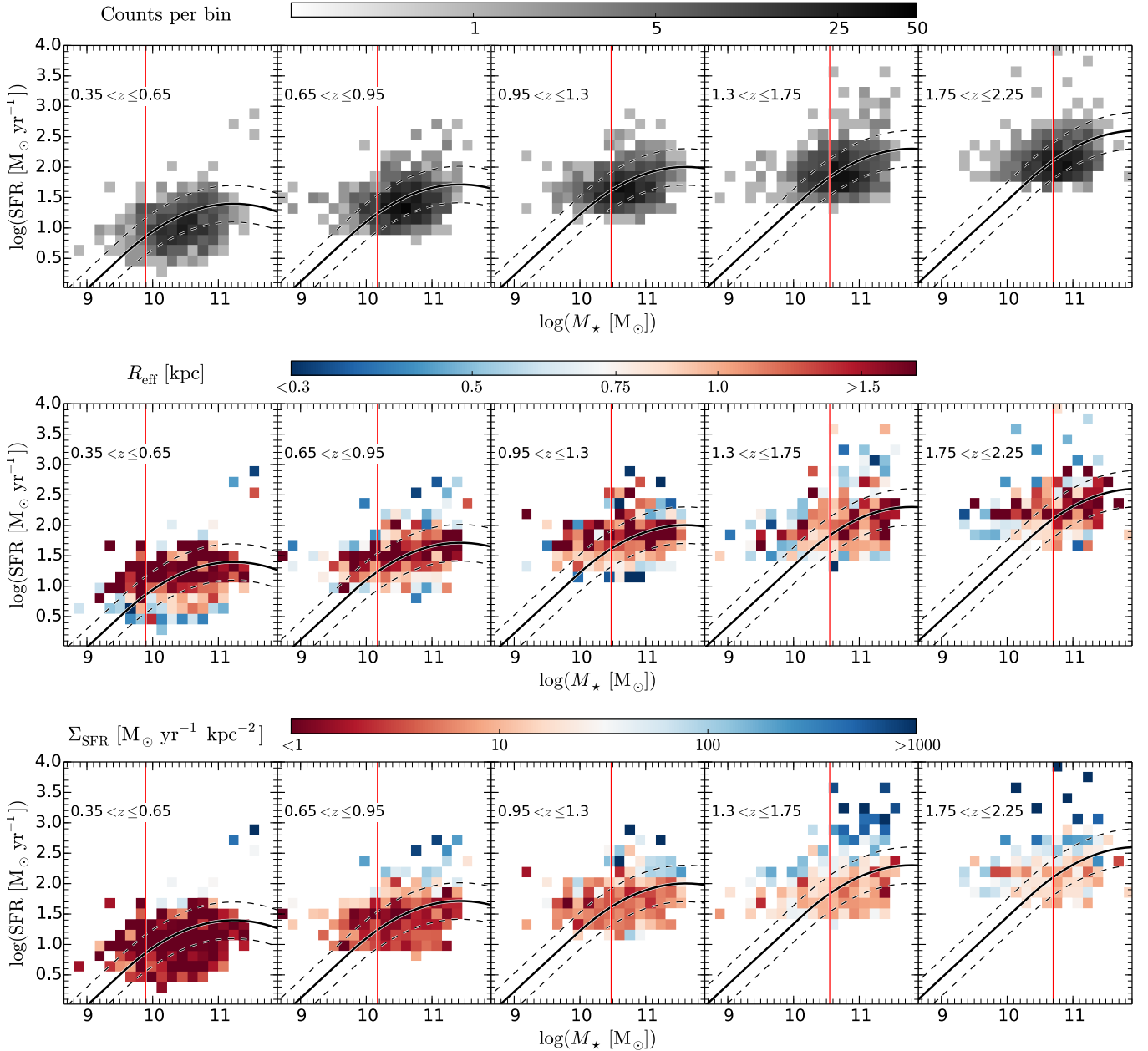
Fig. 6. Upper panels: sample of 3184 SFGs in the SFR– M_* – z plane, color-coded for the number of sources per bin. Shown are the positions of the MS of SFGs (black lines) and the associated dispersion (dashed black lines) given by Schreiber et al. (2015). Vertical red lines show the mass limit above which we consistently probe SFGs on and above the MS. Middle and lower panels: median size and star formation surface density, respectively, of the 3184 SFGs in the sample. We use 1000 MC realizations to include the values for unresolved sources, which are drawn from the distributions described in Sects. 4.2 and 4.4.
