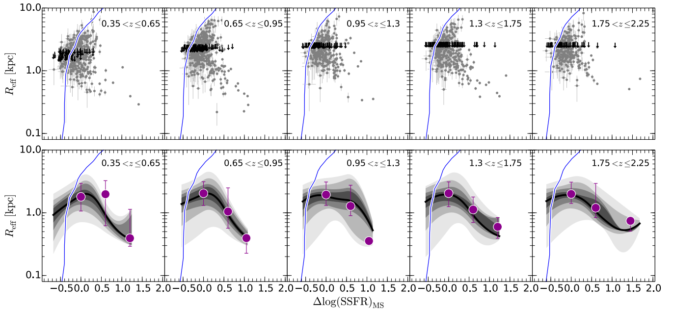
Fig. B.3. Upper panels: star-forming galaxies with M_* > M_*^{\text{lim}} in the size- \Delta \log(\text{SSFR})-z plane. The blue solid line shows the maximum size, corresponding to the 10% completeness level, that can be observed for a galaxy with M_* = M_*^{\text{lim}} evaluated at the central redshift value per bin. Black arrows show the upper limits for the size of unresolved sources. Lower panels: density distribution per \Delta \log(\text{SSFR}) bin (0.5 dex width) of SFGs in the size- \Delta \log(\text{SSFR})-z plane. Contour levels are at the 10, 20, 30, 40, 50, 60, 70, 80, and 90th percentiles. The median size derived via the KM estimator is shown by the dark magenta circles; the error bars correspond to the 16th and 86th percentiles of the distribution.
