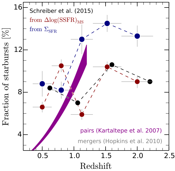
Fig. 13. Redshift evolution of the starburst fraction from the mass-complete sample of radio-selected SFGs used in this work. We adopt two definitions of a starburst galaxy, (a) systems with \Delta \log(\text{SSFR}) > 0.39 and (b) \Sigma_{\text{SFR}} > \Sigma_{\text{SFR}}^{\text{lim}} (see Sect. 5.1), in both cases \log(M_*/M_\odot) > 10.5 . For comparison, we present the starburst fraction for \log(M_*/M_\odot) > 10.5 and \Delta \log(\text{SSFR}) > 0.39 UV/FIR-selected SFGs from Schreiber et al. (2015). The redshift evolution of the observed galaxy pair fraction is shown by the magenta shaded region (Kartalpe et al. 2007). The gray region shows the major merger fraction predicted by Hopkins et al. (2010).
