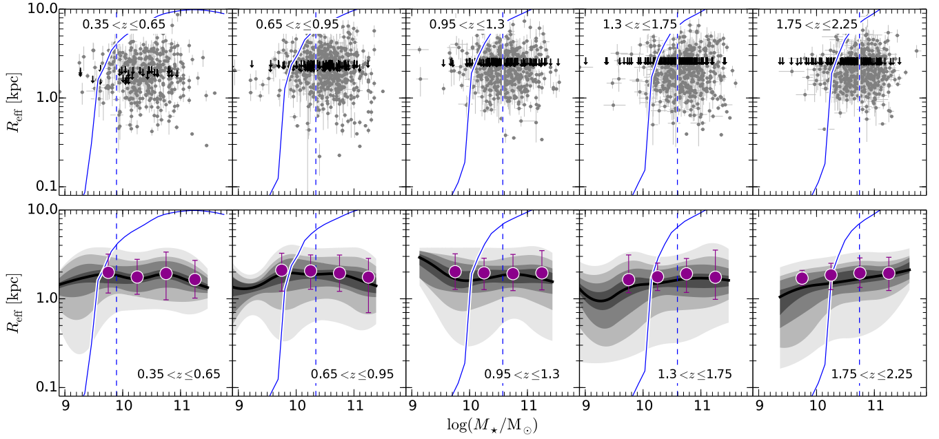
Fig. B.2. Sample of 3184 SFGs in the R_{\text{eff}}-M_* - z plane. The blue solid line shows the maximum size, corresponding to the 10% completeness level, that can be observed for a galaxy with \Delta \log(\text{SSFR}) = 0 evaluated at the central redshift value per bin. Blue dashed lines show the mass-limit above which we consistently probe SFGs on and above the MS. Black arrows show the upper limits for the size of unresolved sources. Lower panels: density distribution per stellar mass bin (0.5 dex width) of SFGs in the R_{\text{eff}}-M_* - z plane. Contour levels are at the 10, 20, 30, 40, 50, 60, 70, 80, and 90th percentiles. The median size derived via the KM estimator is shown by the dark magenta circles; the error bars correspond to the 16th and 86th percentiles of the distribution.
