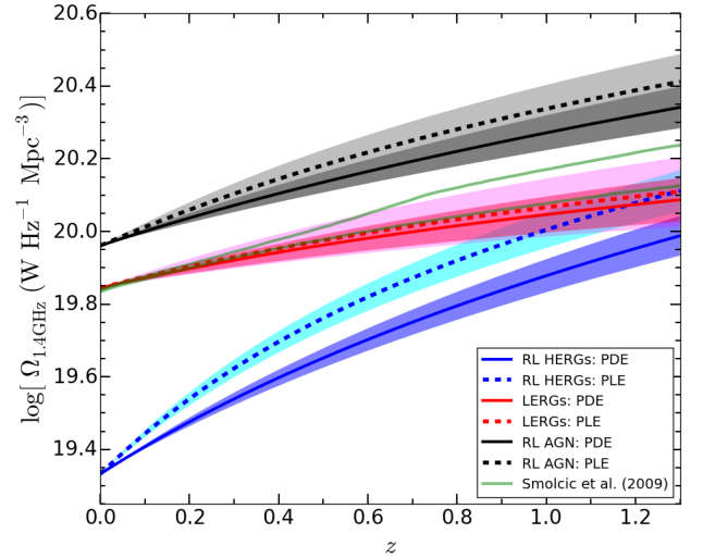
Fig. 17. Evolution of the 1.4 GHz comoving luminosity density ( \Omega_{1.4\text{GHz}} ) for RL HERGs (blue lines), LERGs (red lines), and all RL AGNs (black lines) in XXL-S, integrated from \log[L_{1.4\text{GHz}} (\text{W Hz}^{-1})] = 22.4 to 27.2 (the full range of luminosities probed in the RLFs) at each redshift for best fit PDE (solid lines) and PLE (dashed lines) models. The red and magenta shaded areas represent the uncertainties for the LERG PDE and PLE fits, the blue and cyan shaded areas represent the uncertainties for the RL HERG PDE and PLE fits, and the black and grey shaded areas represent the uncertainties for the RL AGN PDE and PLE fits, respectively. The light green lines represent \Omega_{1.4\text{GHz}} for the low luminosity ( L_{1.4\text{GHz}} < 5 \times 10^{25} \text{ W Hz}^{-1} ) radio AGN in COSMOS from Smolčić et al. (2009).
