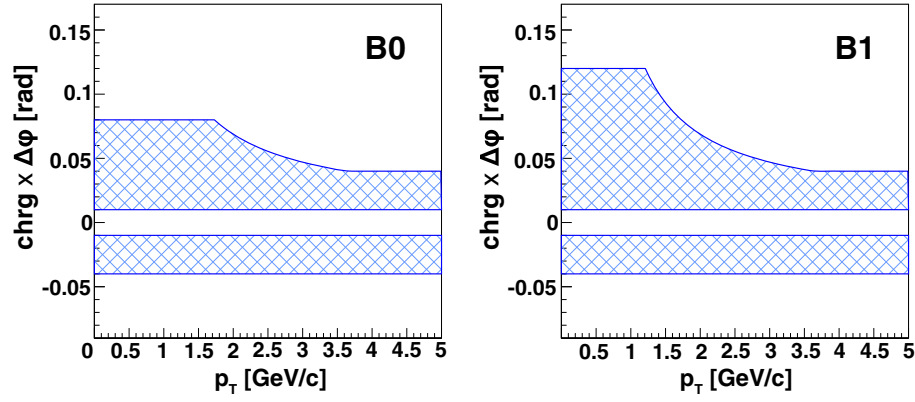
FIG. 5. Track p_T -dependent window in \text{chrg} \times \Delta\phi used in the conversion veto cut in the pixel detector layers, where \text{chrg} is the charge of a given track and \Delta\phi is the azimuthal separation between clusters, one of which is associated with the track.
