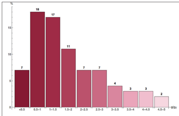
Fig. 4. Distribution of the gravitational constant g among confirmed exoplanets. 19 The values displayed are rounded-off percentages of the total number of sub- 5g_{Earth} exoplanets made up by exoplanets in a given range of surface gravity.
