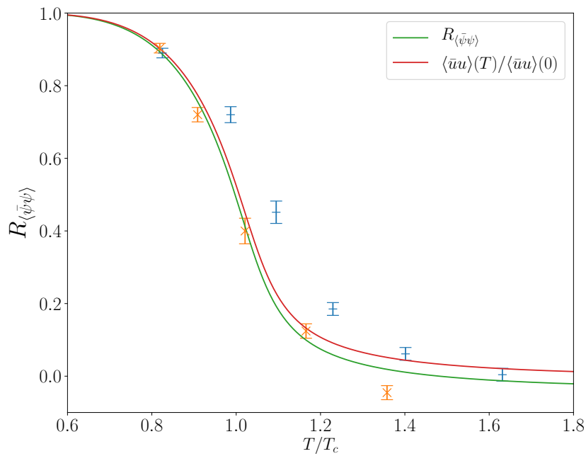
Figure 3. The relative-temperature T/T_c dependence of the subtracted (and normalized) condensate R_{\langle \bar{\psi}\psi \rangle} defined by Equation (17) and introduced by Ref. [81]. The lattice data points are from Figure 6 of Ref. [82], but scaled for the critical temperatures T_\chi from their Table 2, which is different for the “crosses” (data points [82] for m_\pi \approx 370 MeV) and “bars” (data points [82] for m_\pi \approx 210 MeV). The lower, green curve results from the R_{\langle \bar{\psi}\psi \rangle} (17) subtraction of our u -quark condensate. The upper, red curve is the T -dependence of our u -quark condensate when regularized in the usual way (see text).
