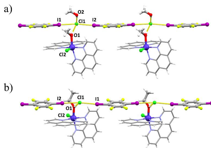
Slika 52. Prikaz povezivanja jedinki halogenskim vezama u lance u kristalnim strukturama koksokratala soli: a) [\text{CoCl}(\text{phen})_2(\text{MeOH})]\text{Cl}(\mathbf{14tfib})(\text{MeOH}) i b) [\text{CoCl}(\text{phen})_2(\text{EtOH})]\text{Cl}(\mathbf{14tfib})
