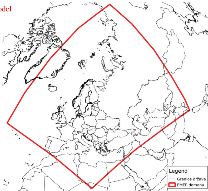
WRF-Chem model
