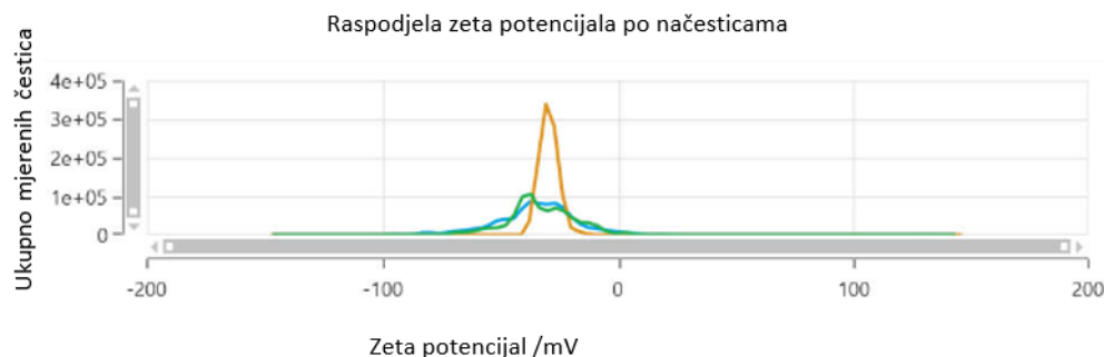
(b) Koloid zlata pomiješan s vodom, -32\text{mV}
