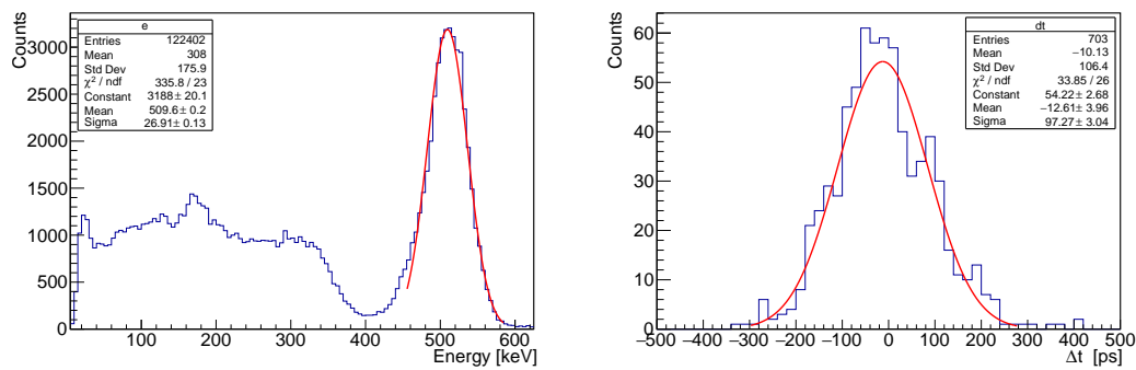
Figure 3. The 511 keV gamma spectrum obtained by 3 \times 3 \times 3 \text{ mm}^3 LYSO crystal with KETEK SiPM at 4 V overvoltage (left). Coincidence time spectrum of annihilation gammas from ^{22}\text{Na} , detected by two 3 \times 3 \times 3 \text{ mm}^3 LYSO crystals with KETEK SiPM at 4V overvoltage (right). Events with energy within 511 \text{ keV} \pm 1 \sigma were selected.
