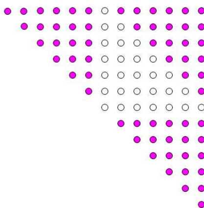
Slika 1.8: T_{2n+1} = 3T_n + T_{n+1}
