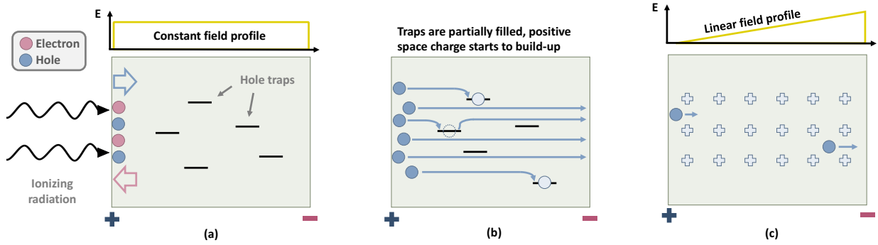
Figure 5.15: Simplified model of polarization effect induced after ionization by short-range radiation in a plane geometry. (a) Radiation impinges the sample and ionizes small volume below the front electrode. Negative bias potential is brought on the back electrode, which attracts holes. Electrons are immediately collected on the positive electrode and do not contribute to the signal. Volume is filled with hole traps. (b) Signal is induced by hole drift, during which some holes are being trapped (and detrapped) on capture centers. As the traps are being filled, positive space charge is building-up throughout the active detector volume. (c) After enough irradiation time, balance of trapping/detrapping rates is established and the created space charge results in a modified electric field profile.
