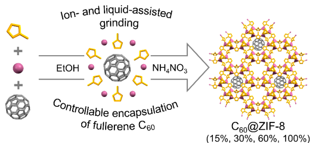
Figure 1. Schematic Representation of the Synthetic Procedure for Encapsulation of Fullerene C 60 into ZIF-8
