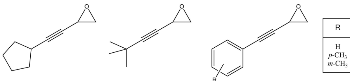
Figure 1. Synthesized propargylic epoxides
