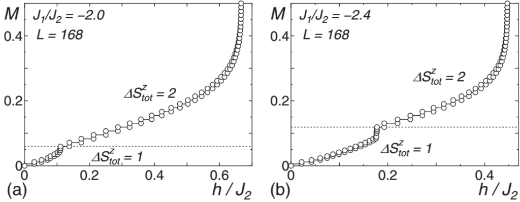
Figure 2.6: Magnetization curves at T = 0\text{K} .
