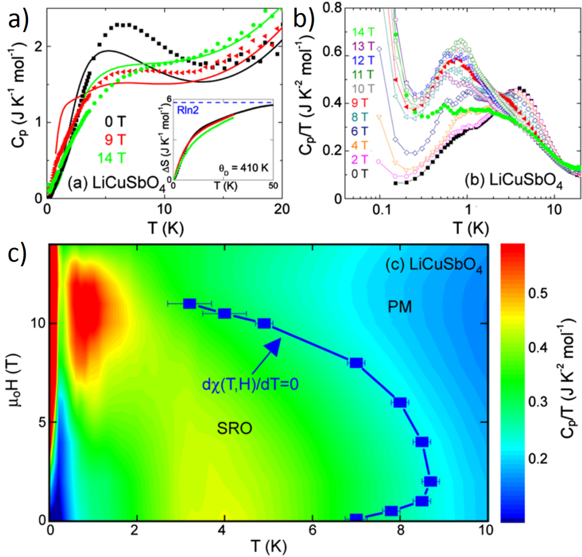
Figure 2.11: Heat capacity measurements on LiCuSbO 4 .
