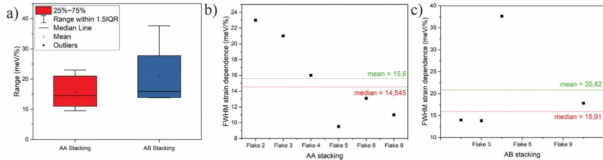
Figure 7.12 a) Comparison of statistical analysis of exciton resonance full width half maximum (FWHM) change with strain for AA and AB stacking. Plotted FWHM strain dependence for AA b) and AB c) stacking for different flakes.
