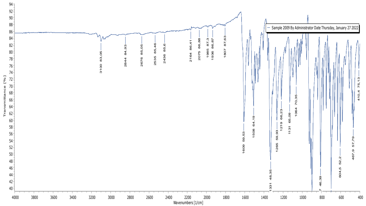
Slika D16. IR spektr [(\text{MoO}_2(\text{L}))_2(4,4'\text{-bipiridin})] .
