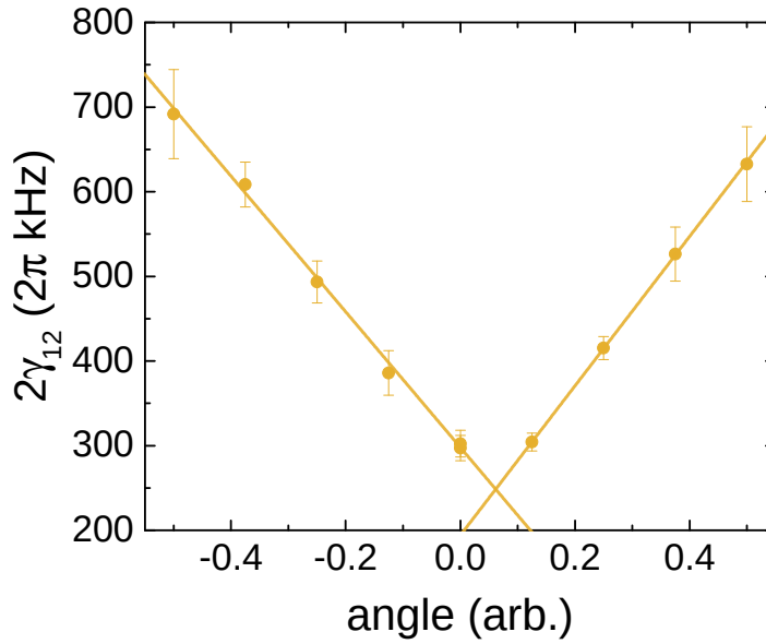
Figure 5.11: Ground state decoherence rate as function of the angle between the probe and the control beam. Crossing of lines marks the minimum intercept, where residual Doppler broadening effect is minimal.
